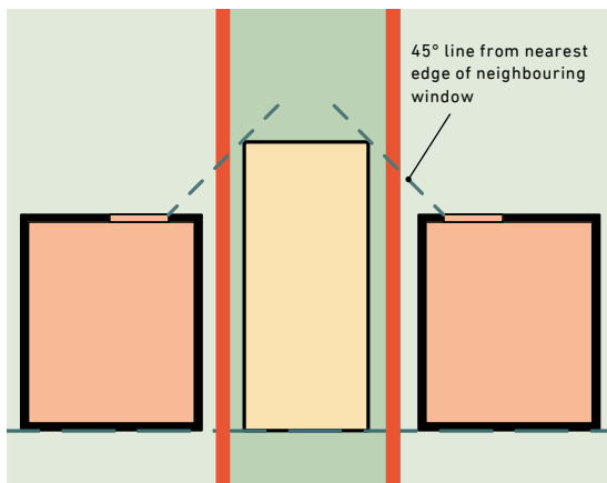
Fig. 101: 45 degree line to limit overbearing of neighbours
