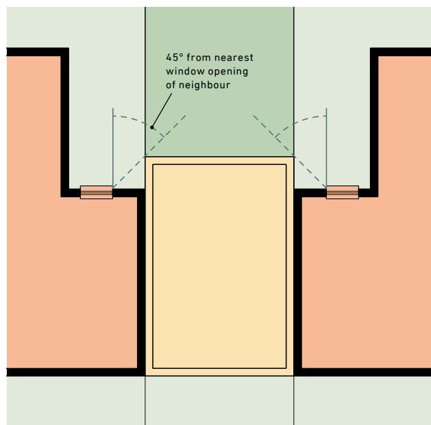
Fig. 116: New development should generally project no further back than a line projected 45 degrees from a neighbouring window
