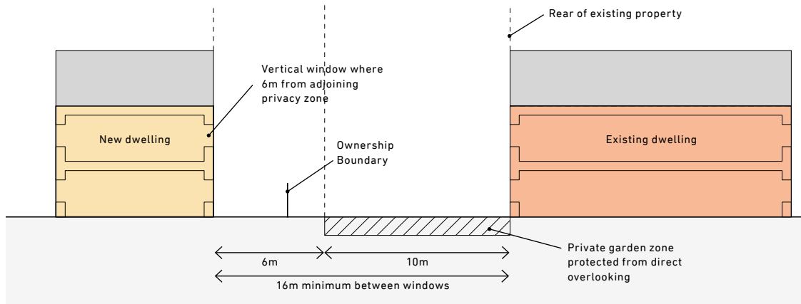
Fig. 29: Conventional windows serving habitable rooms in new dwellings should be at least 6m from the 10m private garden zone
