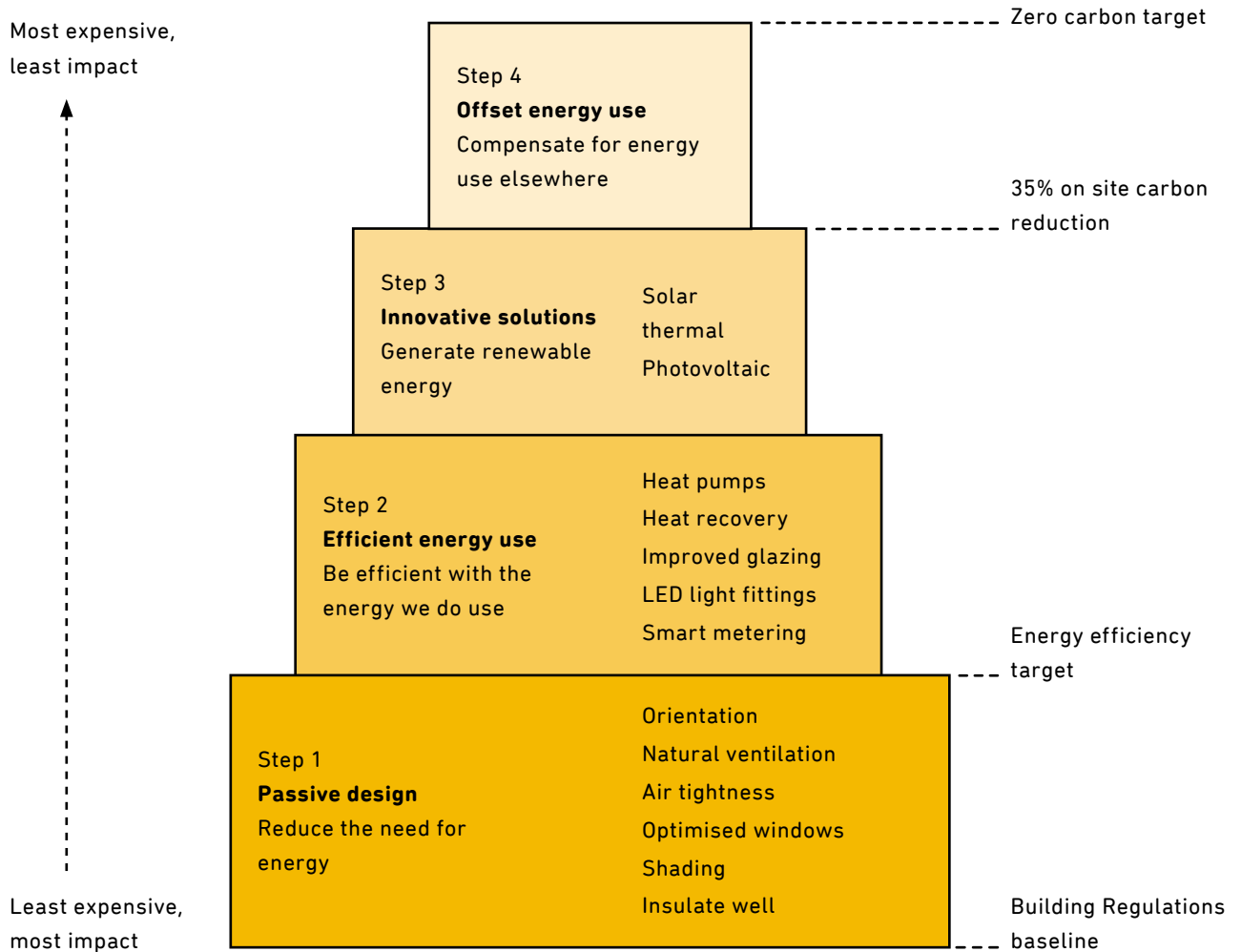
Fig. 80: The Small Sites Energy Pyramid, demonstrating that the least expensive energy-saving methods are the most effective, and increasing capital investment often results in diminishing returns.
