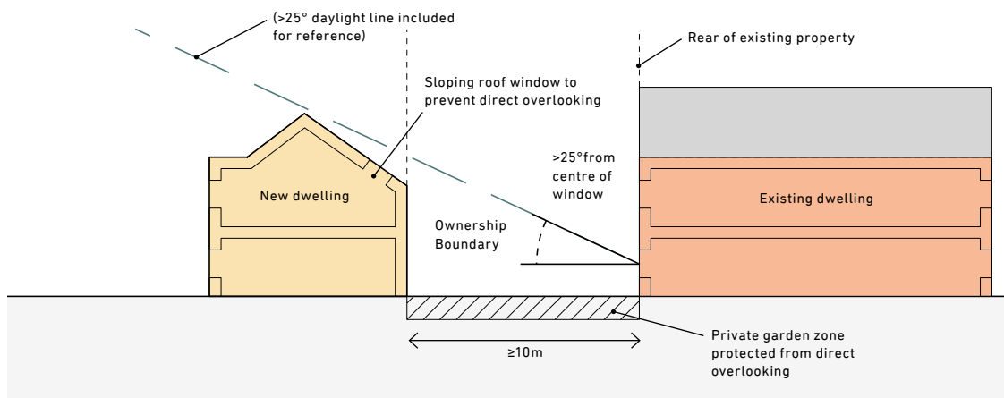
Fig. 31: The use of sloping roof windows can help avoid direct overlooking of neighbouring gardens
