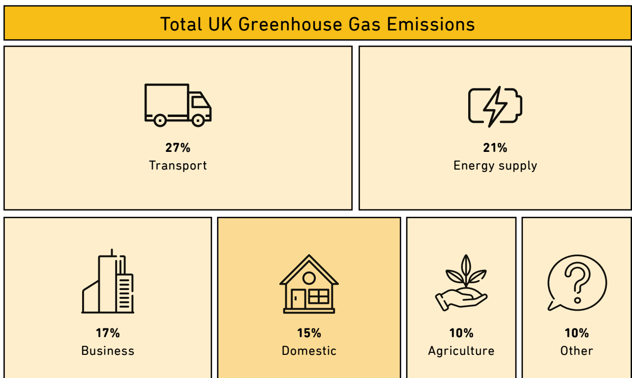
Fig. 78: Diagram showing the sectors responsible carbon emissions across the UK
