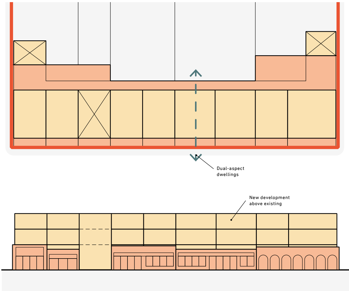
Fig. 166: The potential height of upward development above non-residential uses will depend upon several factors, including structural loading capacity, daylight and overshadowing and access. The creation of residential lobbies within primary frontages is encouraged.
