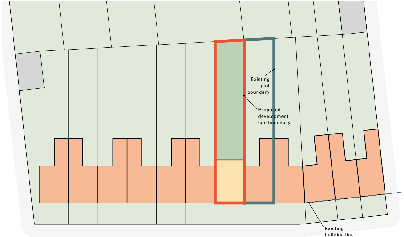
Fig. 117: The sub-division of an existing plot within a terraced street into two can create the opportunity for the construction of a new home.
