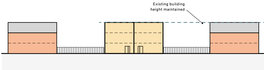
Fig. 154: Where two existing properties have back-to-back gardens, there exists the potential for two new dwellings to be provided.
