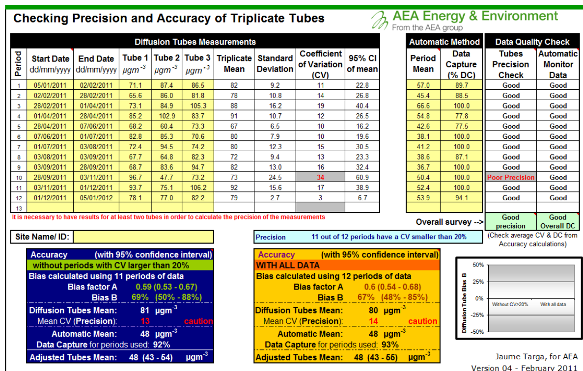
Figure A1: Diffusion tube precision and accuracy, Lewisham 2 collocated
