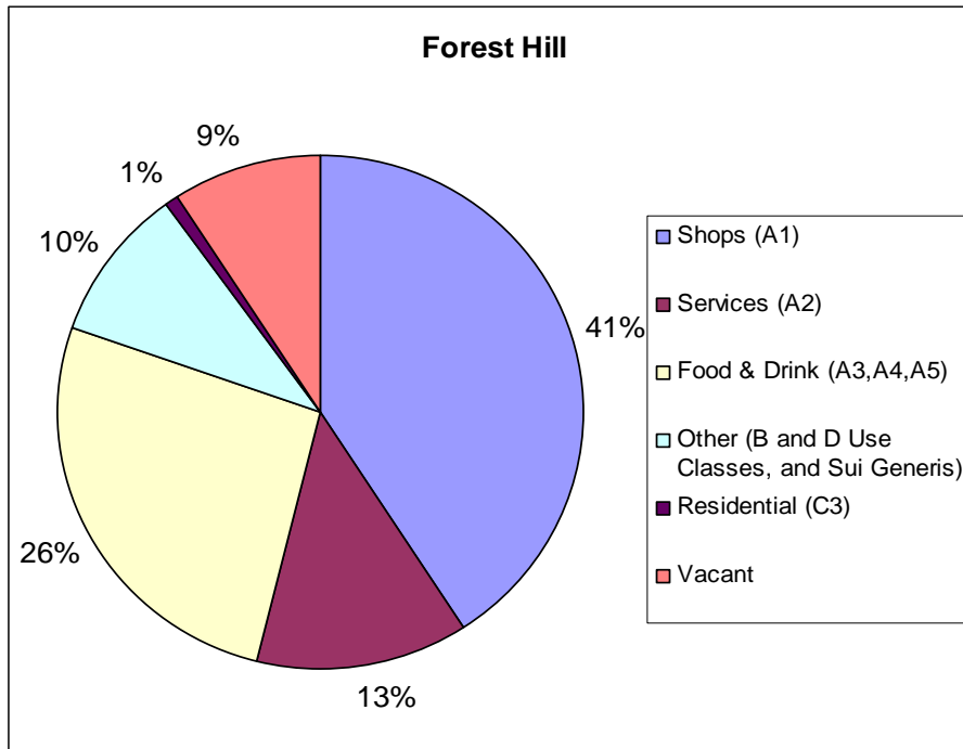
Figure 10: Proportion of units by use class grouping, Forest Hill Town Centre 2013
